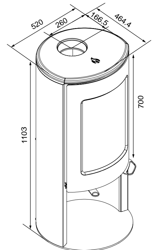
Displayed: WOODSTACKER Size: 520(w) x 465(d) x 1103(h)mm
